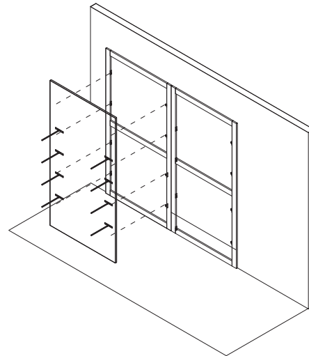
_2 Hook the wall panel with the shelf support through the pre-installed frame supports and the corresponding ones pre-installed on the panel.
