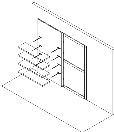
_3 Place the shelf
