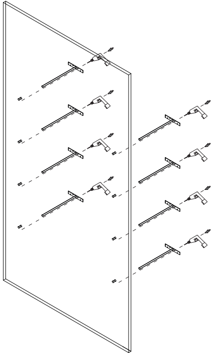
_1 Screw the retractable shelf support to the panel.
